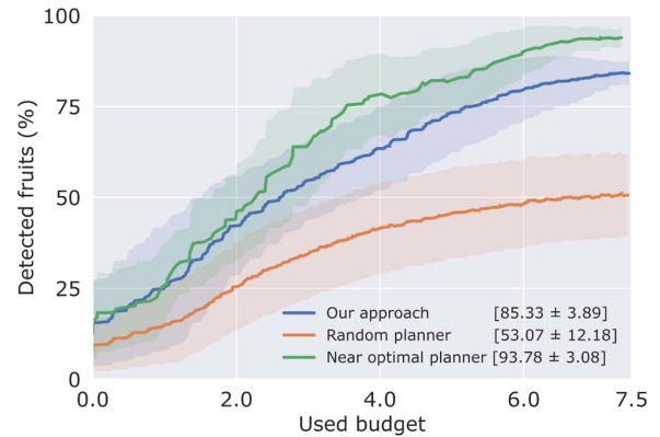
Fig. 6. Comparison of our reinforcement learning-based approach against baselines in a photorealistic fruit monitoring simulator. Solid lines indicate means over ten trials and shaded regions show standard deviations. Our approach performs almost as well as the near-optimal baseline, despite being trained in different environments and not relying on ground truth knowledge.
